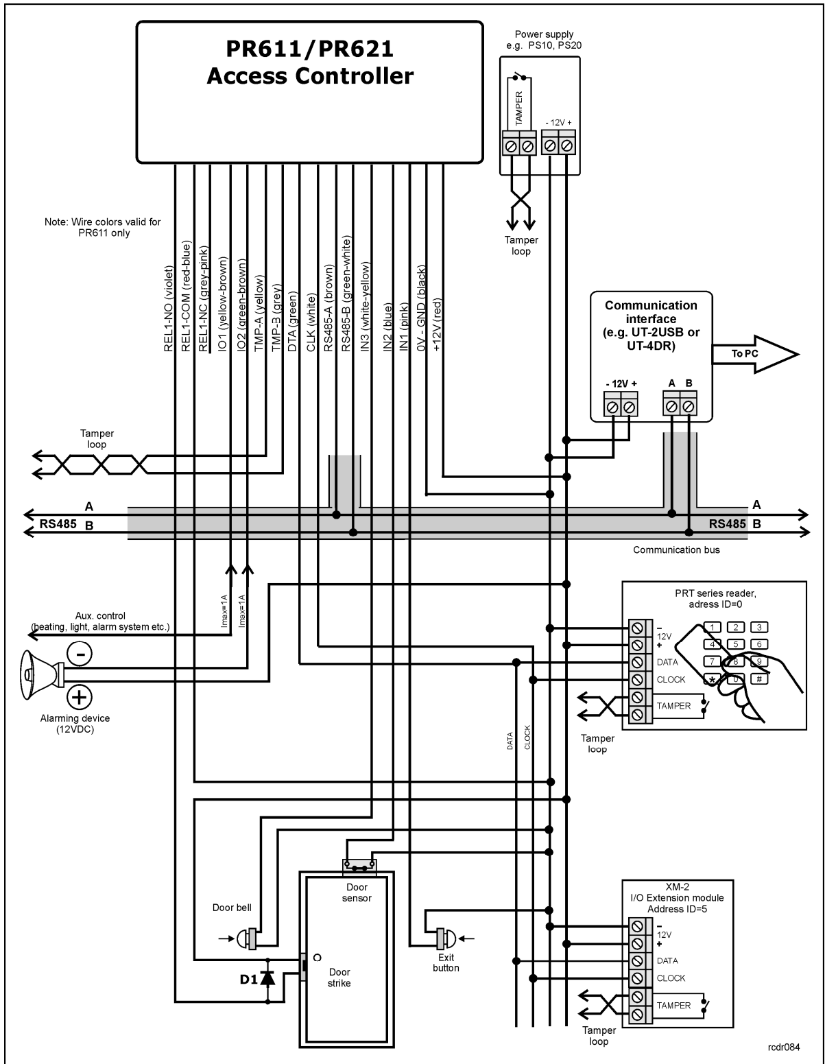
Fig. 1 PR611/PR621 connection diagram
