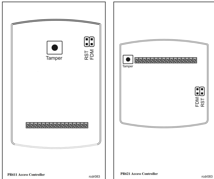
Fig. 6 Location of FDM and RST contacts inside the enclosure of PR611/PR621 controller
